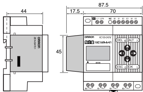
With Battery Unit Mounted
