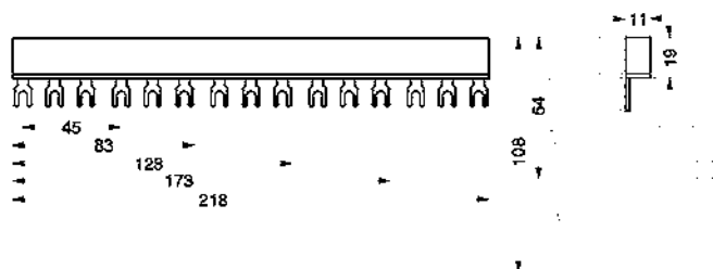
3-phase busbar J74MN-L3-□/□ for J7MN-12 and J7MN-25, modular spacing 45 mm
