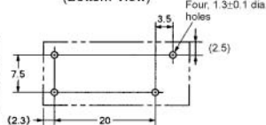
Mounting Hole (Bottom View)
