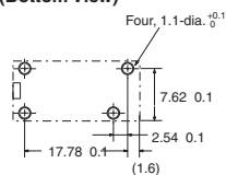
Mounting Holes (Bottom View)
