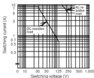
Max. Switching Capacity G5LB-1
