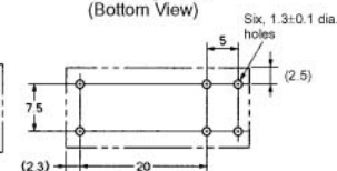
Mounting Holes (Bottom View)
