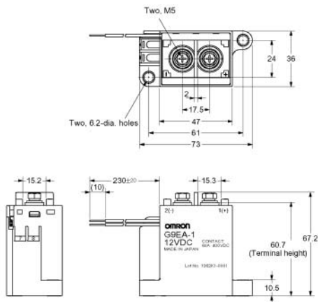
Mounting Hole Dimensions (TOP VIEW)
