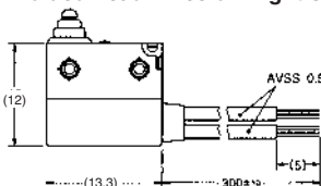
Molded Lead Wires on Right-side
