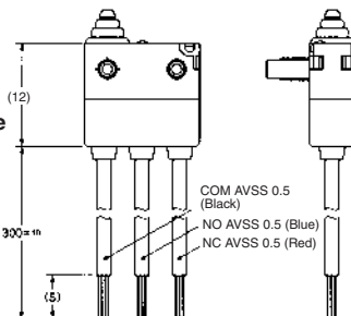
Molded Lead Wires Downwards
