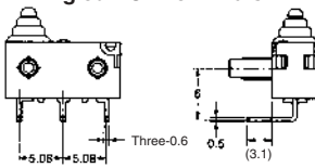
PCB Cutout Dimensions (Reference)
