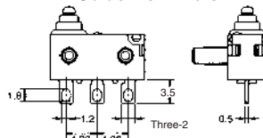
Solder Terminals
