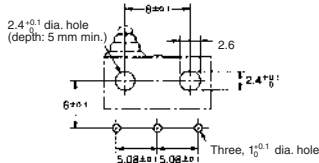
Molded Lead Wires on Right-side
