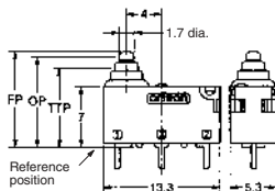
D2HW-A □ Models without Posts
