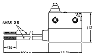
Molded Lead Wires on Left-side
