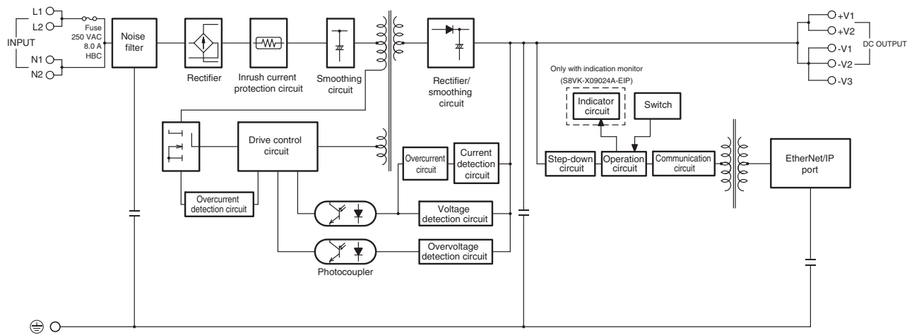
S8VK-X12024-EIP
