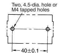
Mounting Holes
